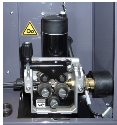
Trainafile a 4 rulli 4-roller wire feeder
